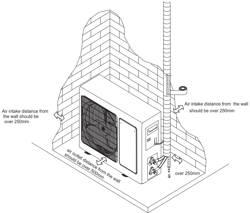
outdoor unit
