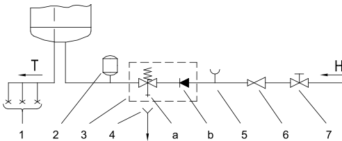
Fig. 2: Closed (pressure) system
