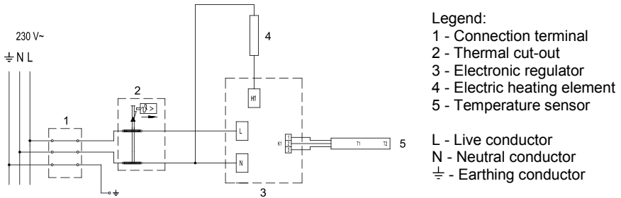
Fig. 5: Electric installation
