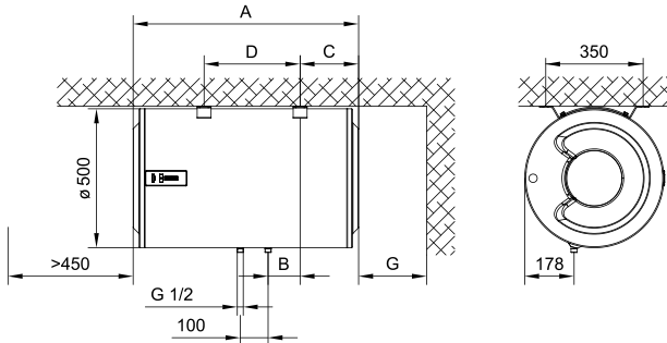
Fig. 1: Horizontal installation on the ceiling
