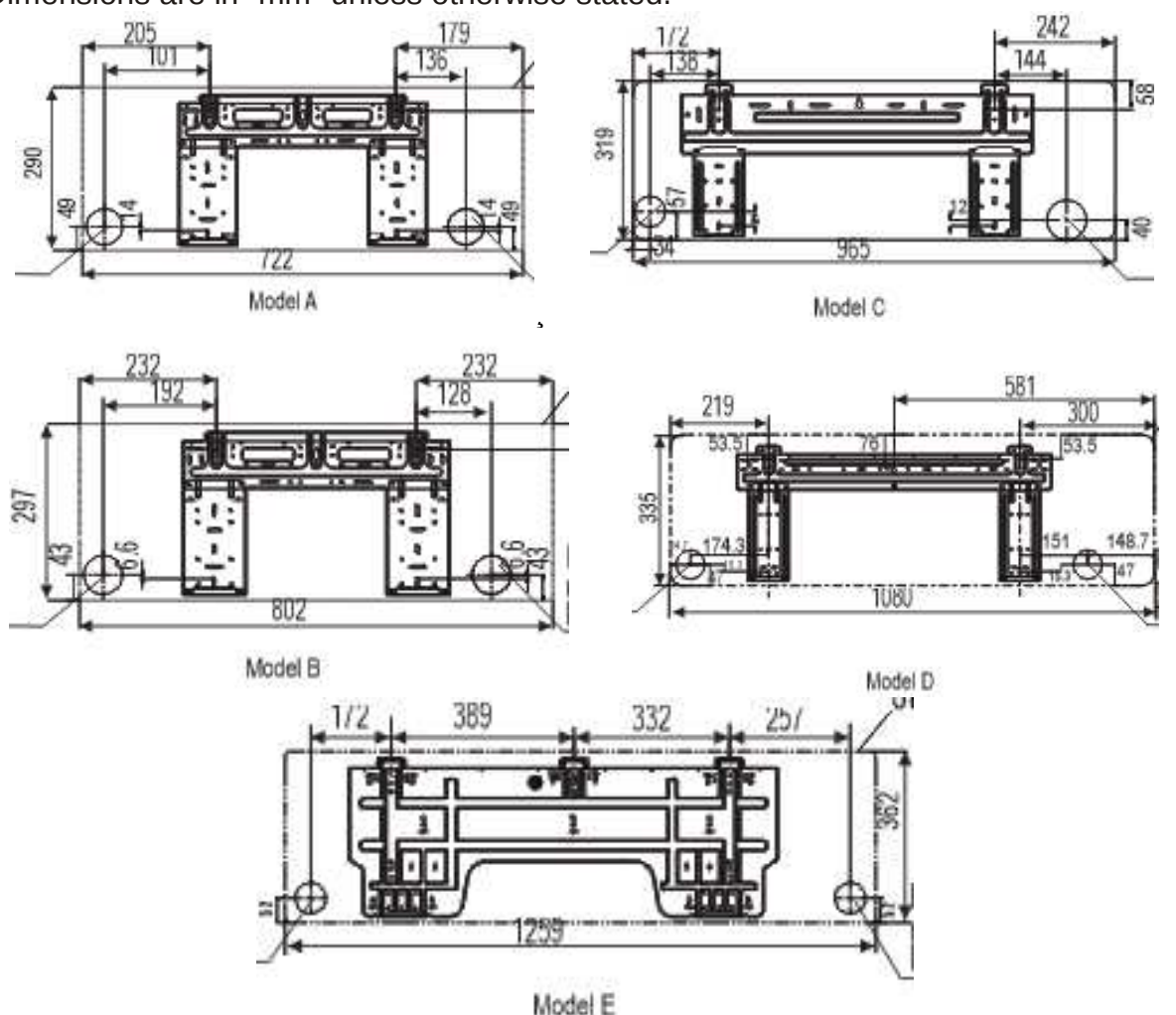
Picture 5: Recommended hole positions for gas pipes and electric wiring KAS26SDCINVA, KAS35SDCINVA, KAS53SDCINVA
