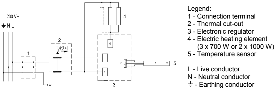
Fig. 5: Electric installation
