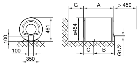
Fig. 2: Montimi horizontal mbi dysheme
