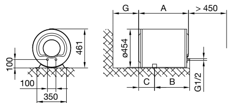
Fig. 2: Horizontal installation on the floor
