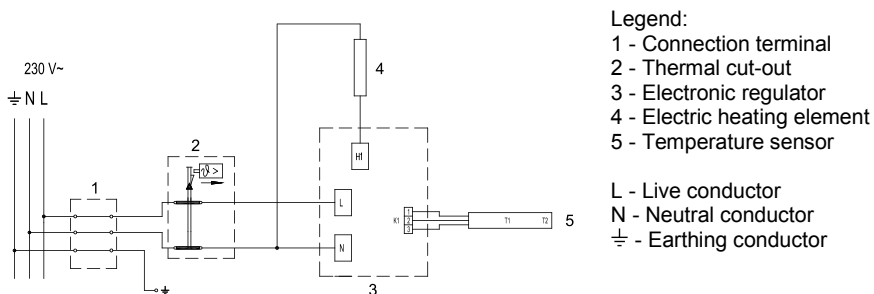
Fig. 5: Electric installation
