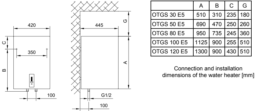
Fig. 1: Vertical installation on a wall
