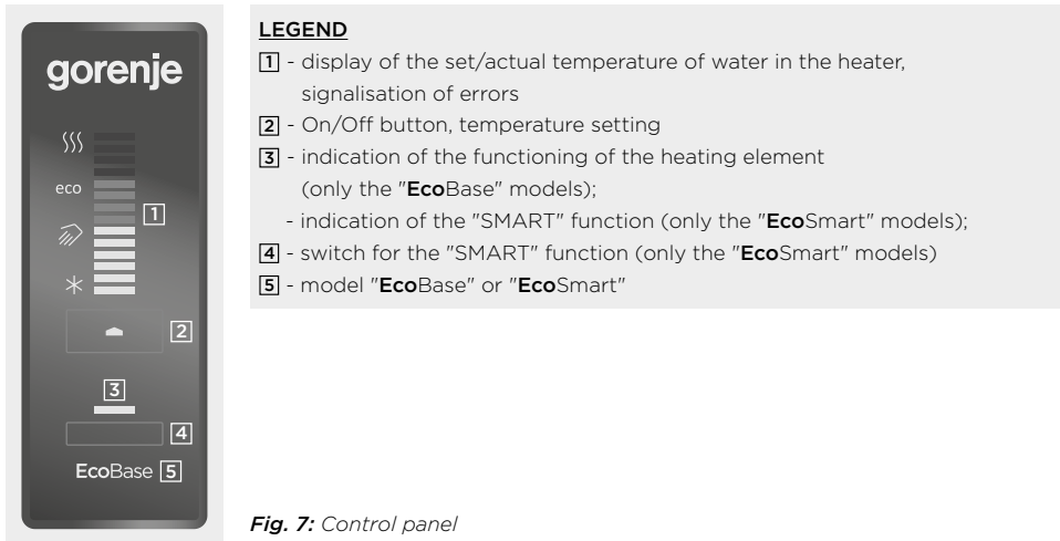
Fig. 7: Control panel
